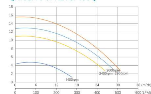
QH.Curve of HLVSP150Q
