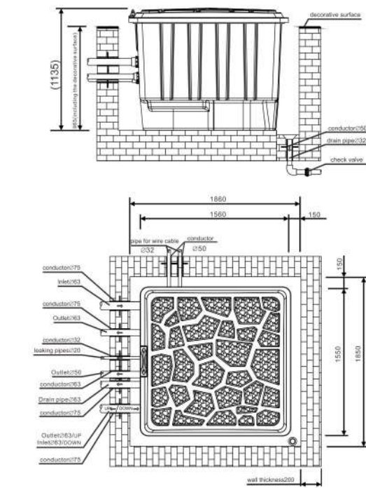
2、WL-GMT-20/25 INSTALLATION DIAGRAM
