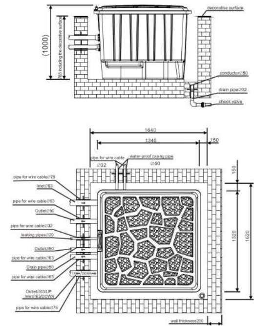
1、WL-GMT-8/12/16 INSTALLATION DIAGRAM
