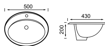
HE-404 Above counter basin Size:500X430X200mm
