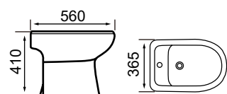
XFH-306 BTW Toilet Size: 560X365X410mm
