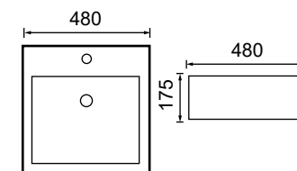
HE-V02 Vanity wash basin Size:480X480X175mm
