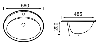
HE-403 Above counter basin Size:560X485X200mm
