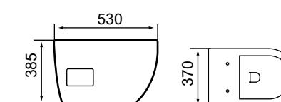
XFH-305 Wall hung toilet Size: 530X370X385mm
