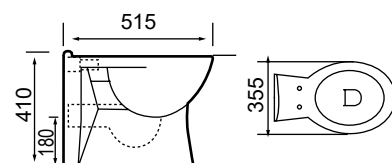
XFH-303 BTW Toilet Size: 515x355x410mm P-trap: 180mm
