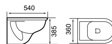
XFH-301 Wall hung toilet Size: 540x360x385mm
