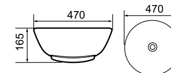
HE-V03 Vanity wash basin Size:470X470X165mm
