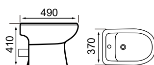
XFH-304 BTW Toilet Size: 490X370X410mm
