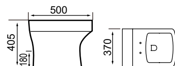
HE-0006K BTW Toilet Size: 500X370X405mm P-trap: 180mm
